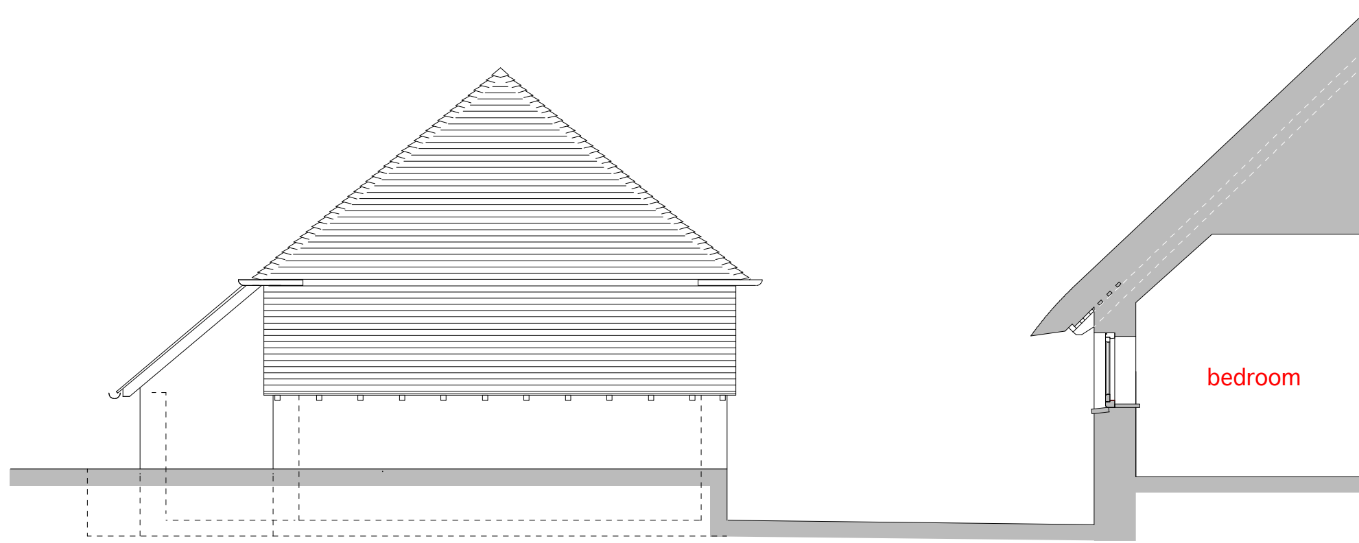
car port - eastern elevation
